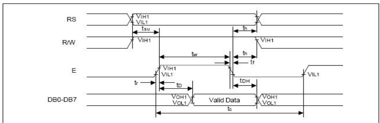
Read Mode Timing Diagram
