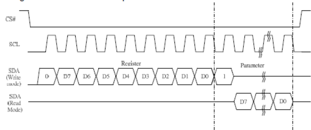
Figure 7-4 Read procedure in 3-wire SPI mode
